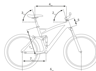
Mercedes-Benz Mountain Bike ALL MOUNTAIN
